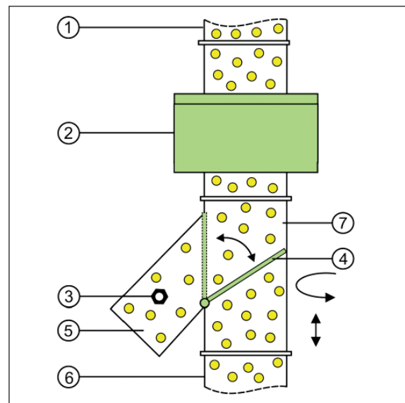
Metal separator RAPID VARIO-FS used for the quality control of PET regenerate.
